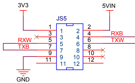
UART Connector
